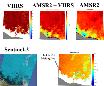
Figure 5: On 18 Jun 2018 over Southeast Hudson Bay. Top: VIIRS, Blended and AMSR2 SIC. Bottom: Sentinel-2 RGB from same day ~17 UTC, and NPP VIIRS IST at 270-275 K scale for same day ~18 UTC.
