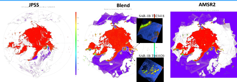
Figure 1: Examples of Daily Sea Ice Concentration Composite over Arctic on 09 Dec 2018. Left: SNPP-VIIRS, Middle: blended VIIRS and AMSR2, Right: AMSR2. SAR-1B images in boxed region over Franz Josef Land and Barents Sea
