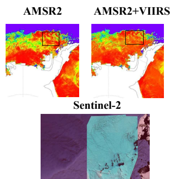
Figure 4: On 15 Oct 2017 over Bellingshausen Sea. Top: AMSR2 and Blended SIC; Bottom: Sentinel-2 RGB from the same day.
