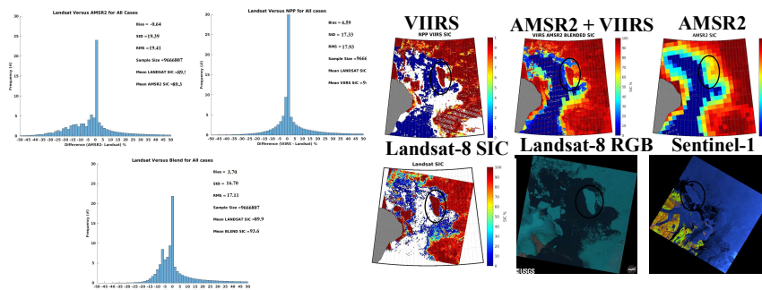
Figure 2: Histogram comparisons to Landsat from 12 Sea Ice Concentration scenes over Arctic from 1 Feb 2017 thru 31 October 2019. Upper left is AMSR2, upper right S-NPP and lower middle is the Blended product.
