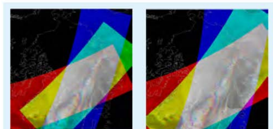
Figure 2. The gray region represents the overlap in three orbits where the polar winds are derived for MODIS (left) and VIIRS (right).
