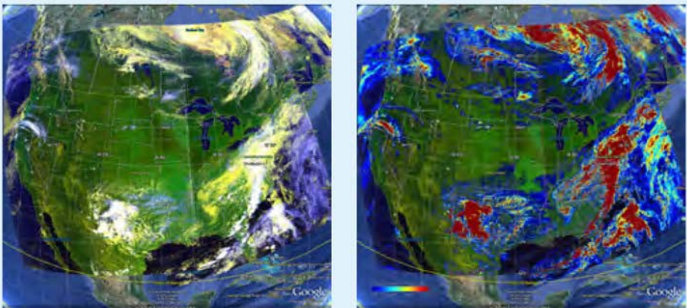
Figure 1. The above images show a result from the Daytime Cloud Optical and Microphysical Properties algorithm. The image on the left is a false color image constructed from the 0.65, 0.86 and 1.1 mm channels. The image on the right shows the cloud water path overlaid onto the false color image. These images are generated using the direct broadcast data from SSEC.
