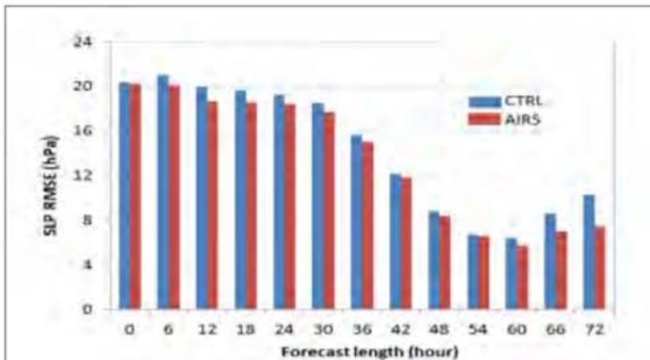
Figure 2. Tropical Cyclone Irene (2011) central sea level pressure (SLP) forecast RMSE for 0-h (analysis), 6-h, to 72-h forecasts. Every 6 hours between 06 UTC 23 and 00 UTC 25 August 2011 the data are assimilated with WRF/DART followed by a 72-hour forecast. The SLP RMSE is calculated from comparisons with the best track observations from National Hurricane Center.
