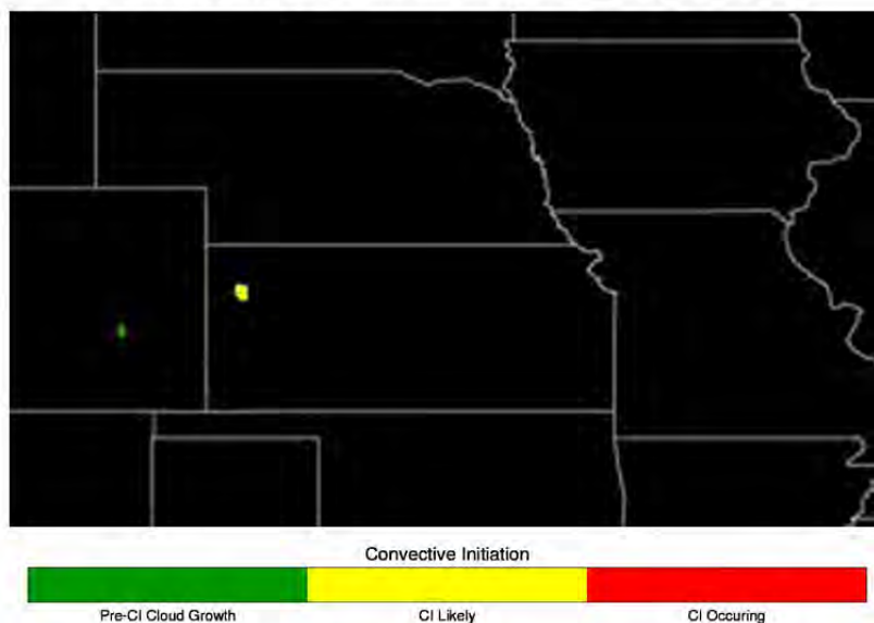
Convective Initiation: 20100610 at 2132 UTC
