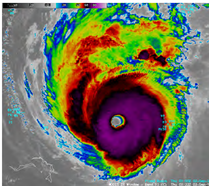
MODIS IR image of Hurricane Earl approaching the US East Coast.
