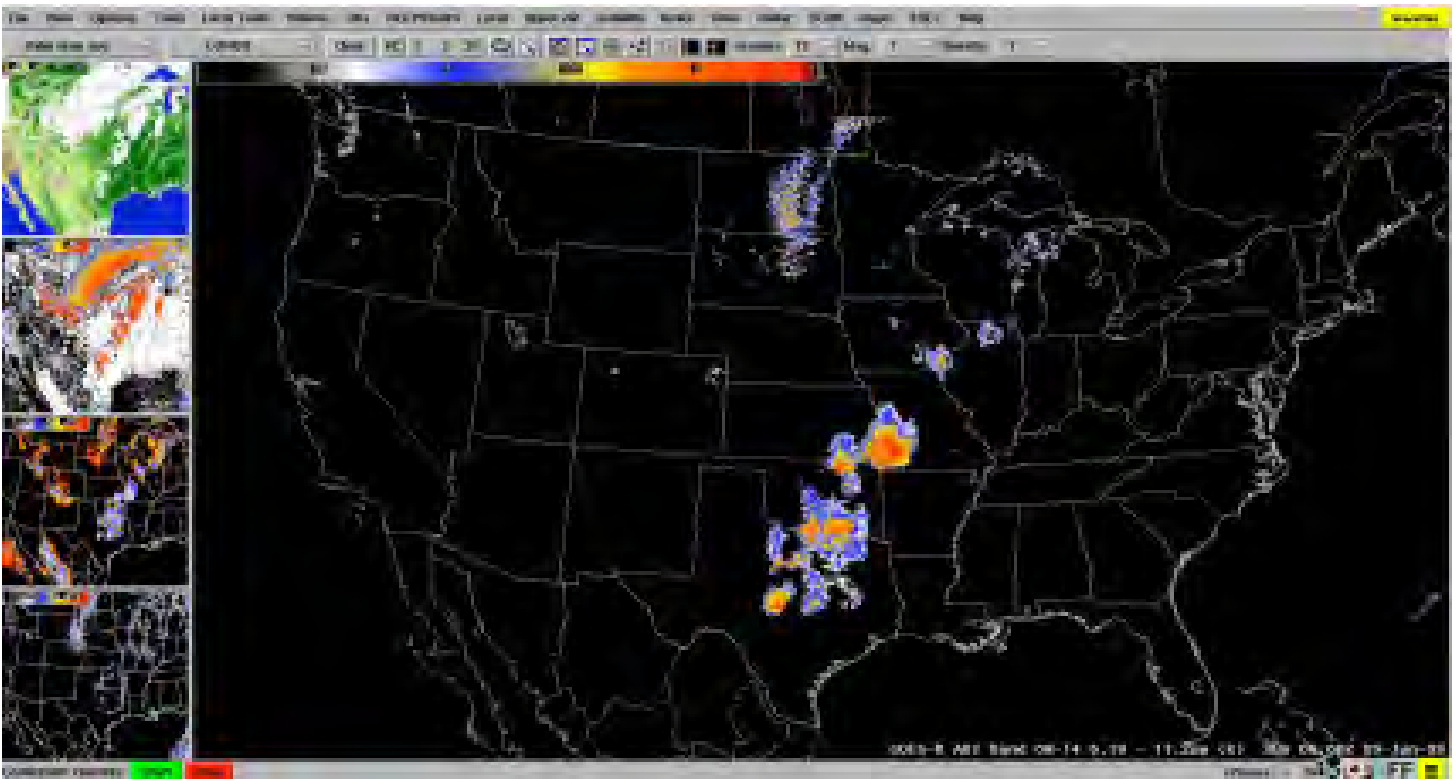
Band differences used to detect areas with the greatest potential for convection.
