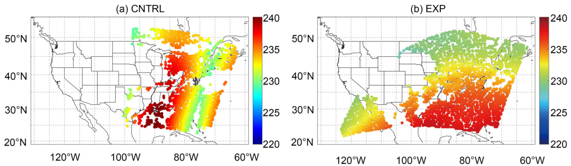
Fig. 7. The assimilated CrIS-FSR channel 97 BT (K) for (a) CNTRL from SNPP and NOAA-20 and (b) EXP from GEO for Case II at 0600 UTC 27 May 2019. The thinning box is 60 km for both experiments.
